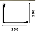
L2 ARSTYL® 200 x 250 x 2000mm
